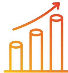
Scalability
